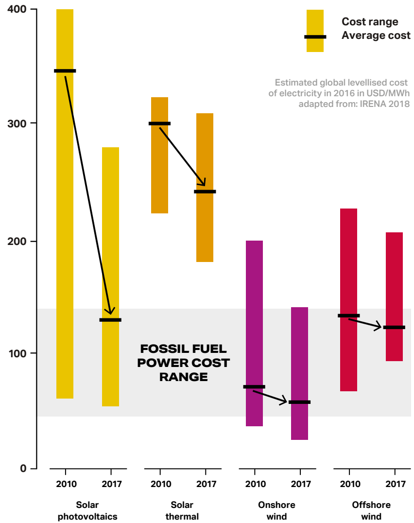
Figure 5. Price drop in solar and wind power since 2010 The dramatic fall in costs of wind and solar energy in the last decade has reached a tipping point where prices increasingly are lower than many fossil fuel alternatives. Source: Irena Renewable Cost Database. 5
