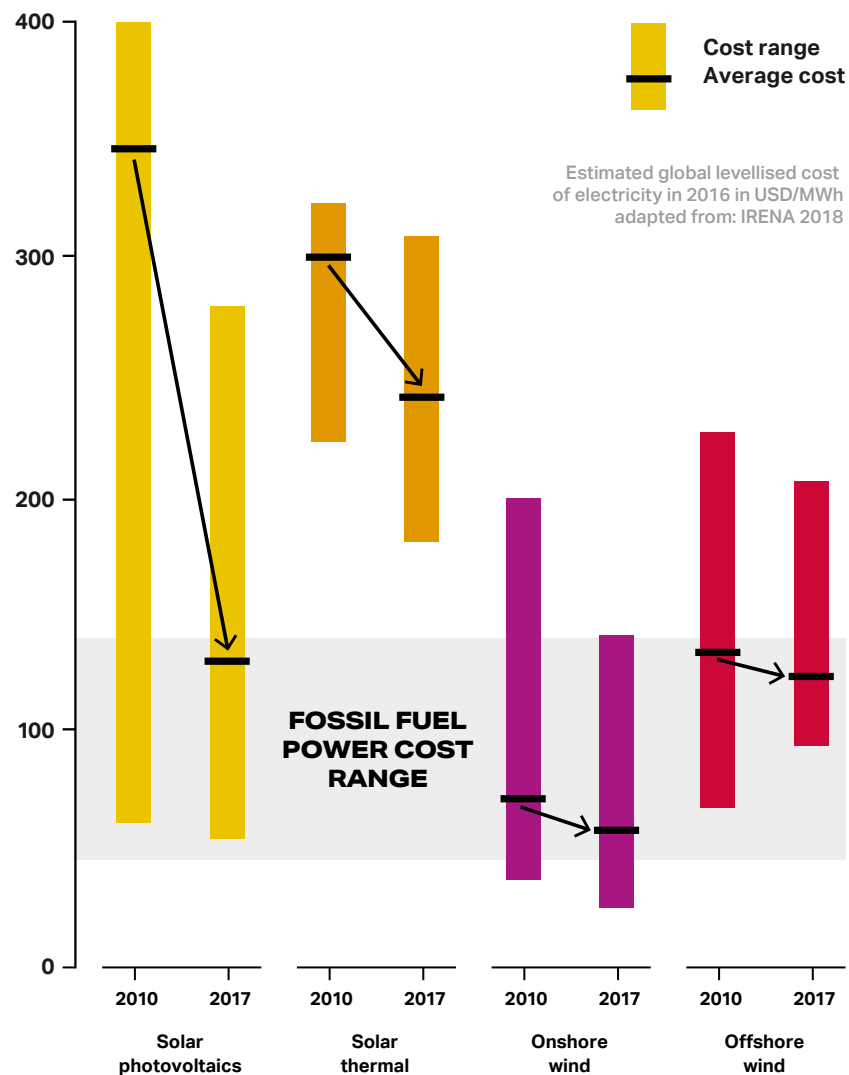
Figure 21. Cost of wind and solar power generation
