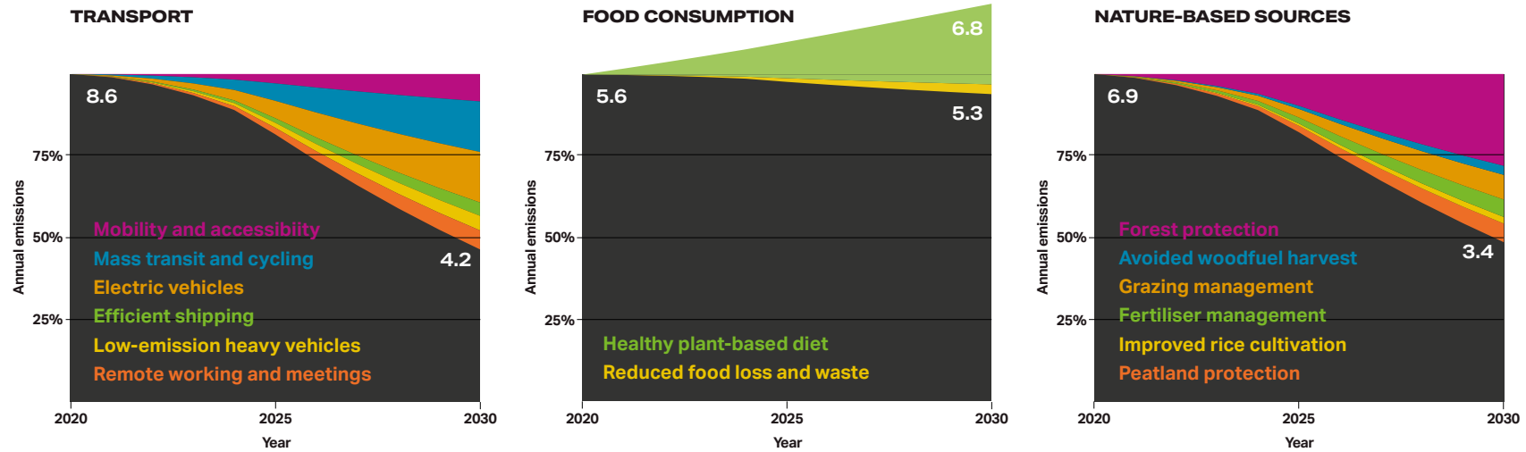
Figure 1. Sectoral roadmap to halve emissions by 2030
