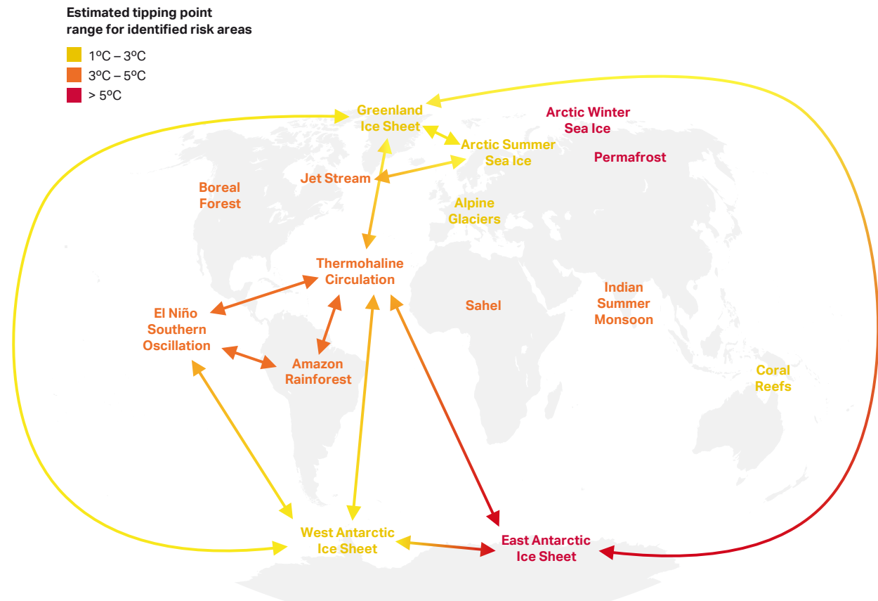
Figure 6. Earth's tipping points
