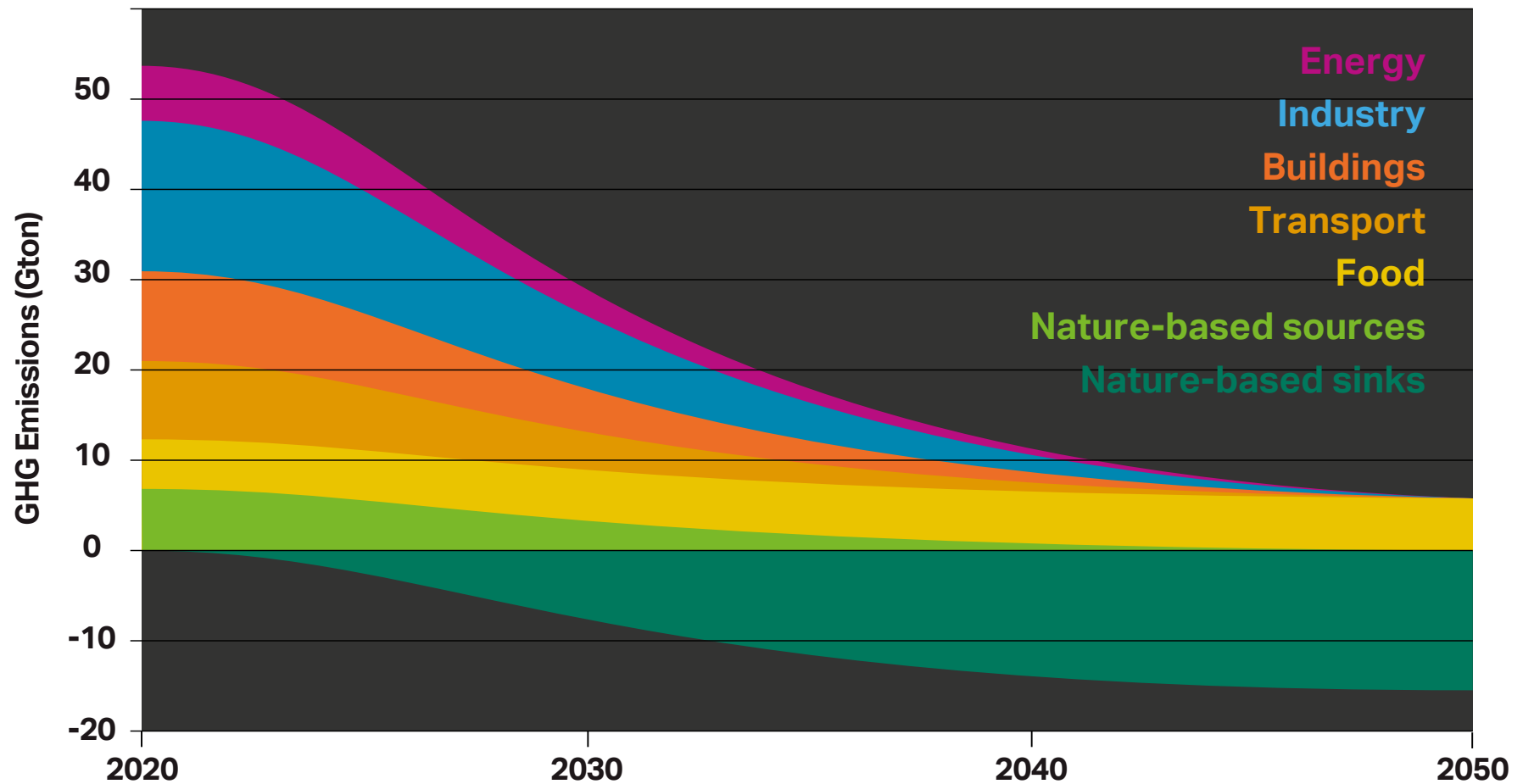
Figure 3. Exponential emission reduction pathways to limit global warming to 1.5°C
